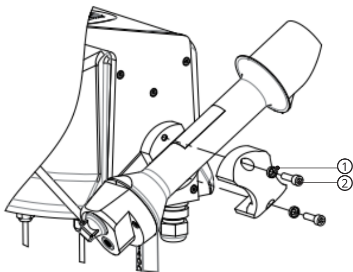
Mounting a SHP1 pyrhelimeter
